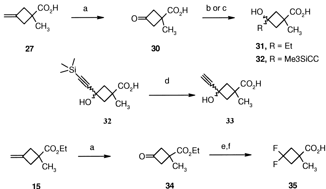
Scheme 6. Preparation of cyclobutane carboxylic acids 31 , 33 and 35 . (a) \text{O}_3 , \text{CH}_2\text{Cl}_2 , then (\text{CH}_3)_2\text{S} , 78%; (b) \text{EtMgBr} , THF, 64%, cis and trans isomers separated by chromatography; (c) lithium TMS acetylide, THF, 85%, cis and trans isomers separated by chromatography; (d) \text{NaOH} , \text{MeOH} , 70%; (e) DAST, \text{CH}_2\text{Cl}_2 ; (f) \text{NaOH} , \text{H}_2\text{O} , 100^\circ\text{C} , 43% (two steps).
