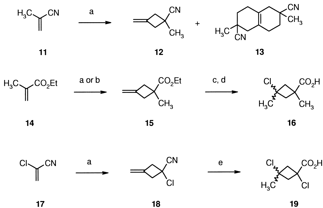
Scheme 2. Synthesis of cyclobutane carboxylic acids 16 and 19 . (a) Allene (1.66 equiv), hydroquinone (catalytic), benzene, 200 °C, 23–30%; (b) allene (0.25 equiv), hydroquinone (catalytic), benzene, 200 °C, 41%; (c) NaOH, H 2 O, 100 °C, quantitative; (d) concd HCl, rt, 77%; (e) concd HCl, 100 °C, 40%.
