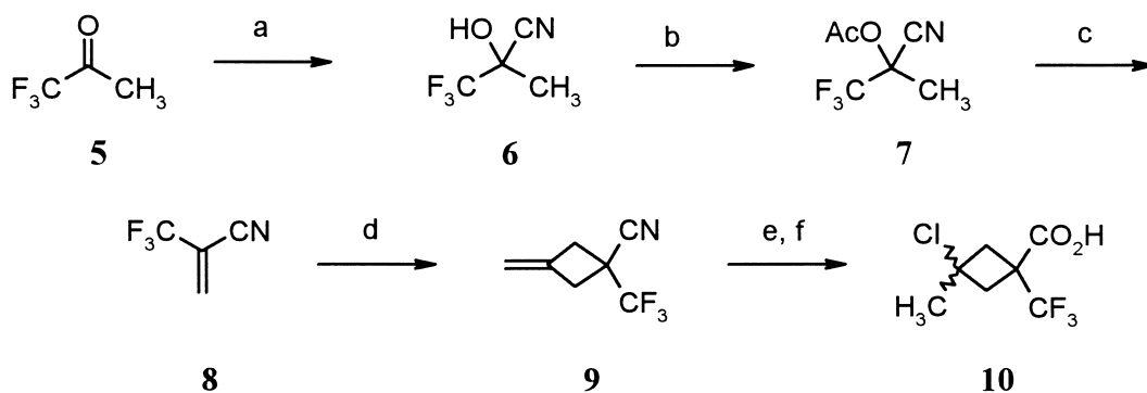
Scheme 1. Synthesis of cyclobutane carboxylic acid 10 . (a) KCN, H 2 SO 4 , 60%; (b) AcCl, reflux, 84%; (c) pyrolysis at 520 °C, 66%; (d) allene (1.6 equiv), hydroquinone (catalytic), benzene, 200 °C, 25%; (e) NaOH, H 2 O, 100 °C, 96%; (f) concd HCl, rt, 68%.
