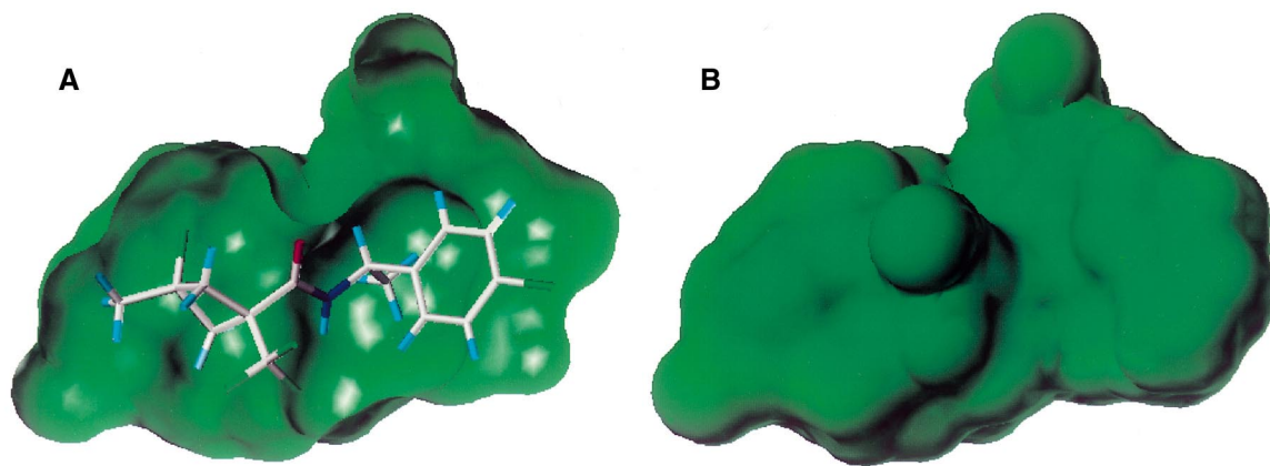
Figure 3. (A) Cross section of the Connolly surface of the SD binding pocket showing 4 . (B) Connolly surface of the SD binding pocket generated from the crystal structure of the SD- 4 .
