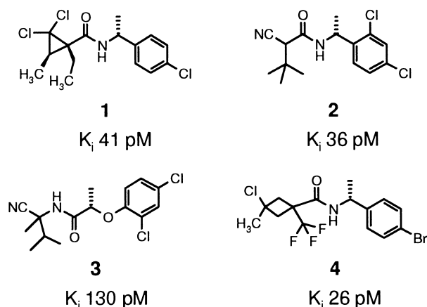
Figure 1. Inhibitors of scytalone dehydratase (SD).
