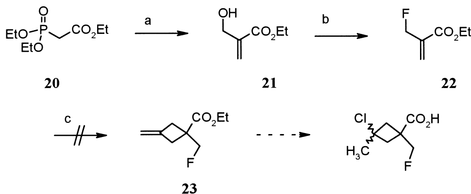
Scheme 3. Attempted preparation of fluoromethyl cyclobutane carboxylic acid. (a) Formaldehyde, \text{H}_3\text{PO}_4 , \text{K}_2\text{CO}_3 , 69%; (b) DAST, \text{CH}_2\text{Cl}_2 , 45%; (c) allene, hydroquinone (catalytic), benzene, 200^\circ\text{C} .
