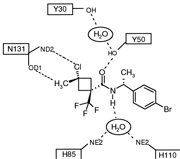
Figure 2. A schematic drawing of the interactions between 4 and SD.
