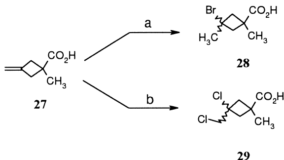
Scheme 5. Synthesis of substituted cyclobutanecarboxylic acids 28 and 29 . (a) HBr, 66%; (b) dichloriodobenzene, \text{CH}_2\text{Cl}_2 , 46%.
