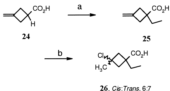
Scheme 4. Preparation of cyclobutane carboxylic acid 26 . (a) LDA, THF, then EtI, 68%; (b) concd HCl, 100%.
